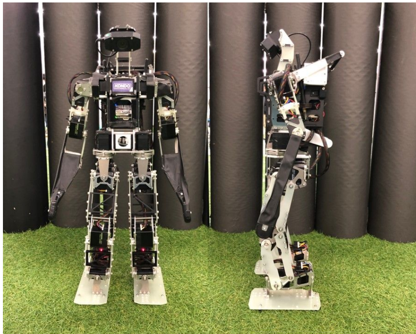
Structure of the GankenKun
