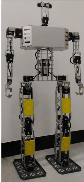
ZSTT-AUT Adult-size Humanoid robot
